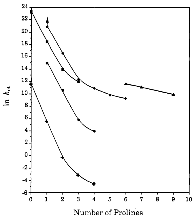
Figure 2. Rates of intramolecular electron transfer across five series of oligoproline donor-acceptor complexes: ▲, \{(\text{bpy})_2\text{Ru}^{\text{II}}\text{L}\}^{\cdot-}(\text{Pro})_n\text{Co}^{\text{III}}(\text{NH}_3)_5\}^{\cdot-} ; ◆, \{(\text{bpy})_2\text{Ru}^{\text{II}}\text{L}\}^{\cdot-}(\text{Pro})_n\text{Co}^{\text{III}}(\text{NH}_3)_5\}^{\cdot-} ; ■, \{(\text{bpy})_2\text{Ru}^{\text{II}}\text{L}\}^{\cdot-}(\text{Pro})_n\text{Co}^{\text{III}}(\text{NH}_3)_5\}^{\cdot-} ; ●, \{(\text{bpy})_2\text{Ru}^{\text{II}}\text{L}\}^{\cdot-}(\text{Pro})_n\text{Co}^{\text{III}}(\text{NH}_3)_5\}^{\cdot-} ; +, \{(\text{bpy})_2\text{Ru}^{\text{II}}\text{L}\}^{\cdot-}(\text{Pro})_n\text{Co}^{\text{III}}(\text{NH}_3)_5\}^{\cdot-} .
